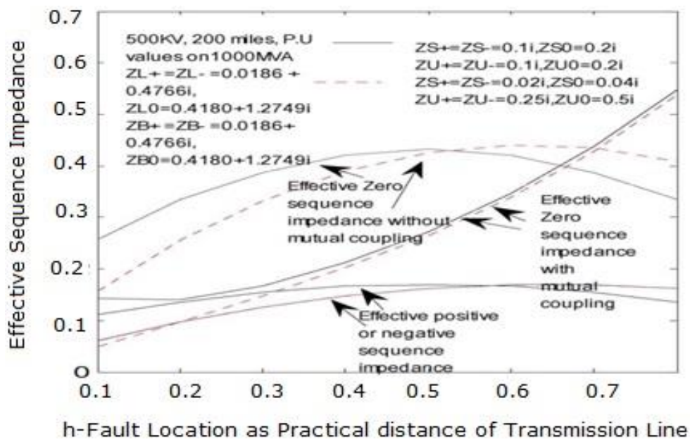
Fig 2. Fault location with effective sequence impedance
