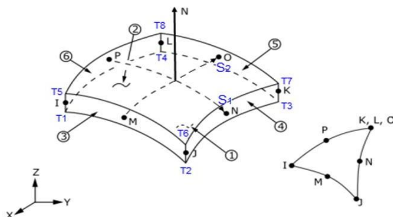
Fig 1: Element coordinate system, the geometry and node locations for Shell 281
