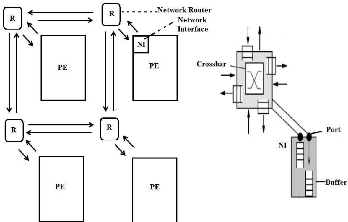
Fig 2. “2D Mesh router and NI details”[3]
