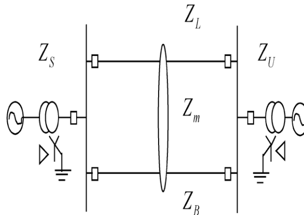
Fig.1. Parallel line (Twin-circuit)
