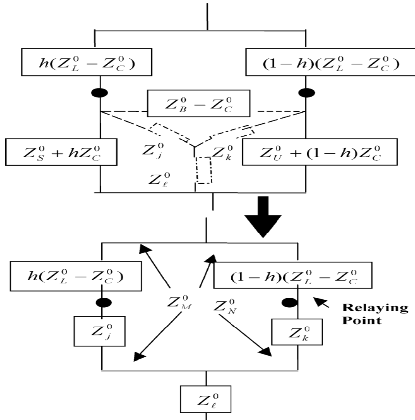
Fig 4. Equivalent Circuit and Inter-Circuit Zero-Sequence Mutual Coupling
