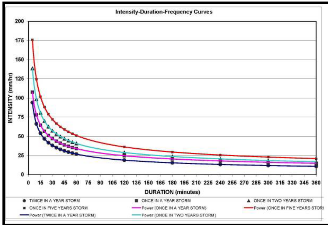
Figure 3. Intensity-Duration-Frequency Curves
