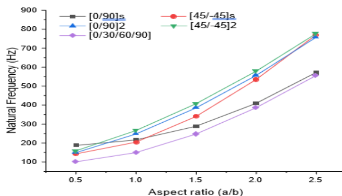
Fig 3. Variation of natural frequency with aspect ratio ( \Delta T = 750^\circ\text{C} )
