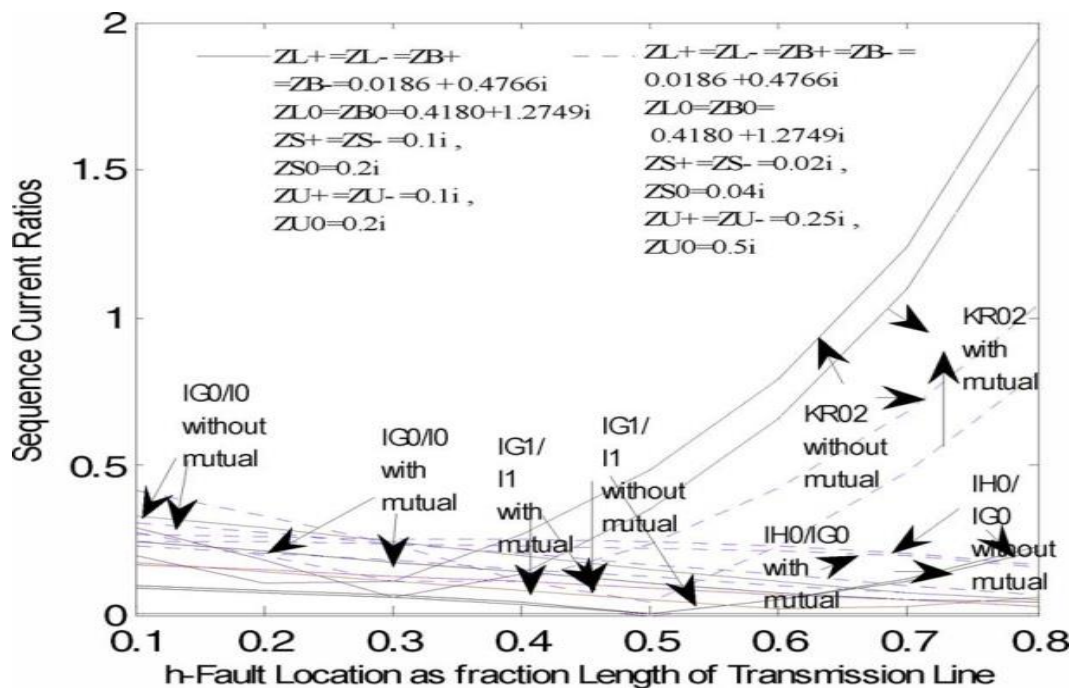
Fig. 3 Fault location and sequence current ratios
