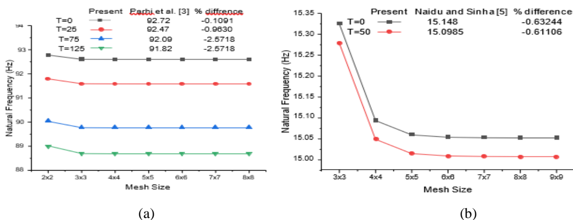
Fig 2: Convergence and comparison of eigen frequency of laminated composite plate
