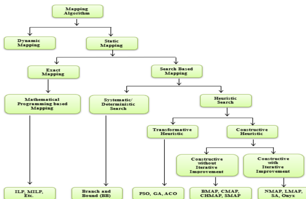
Fig 3. Classification of mapping algorithms [2]
