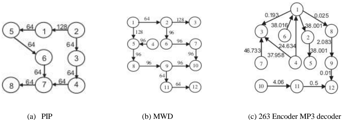
Fig 1. shows various types of Task Graphs.
