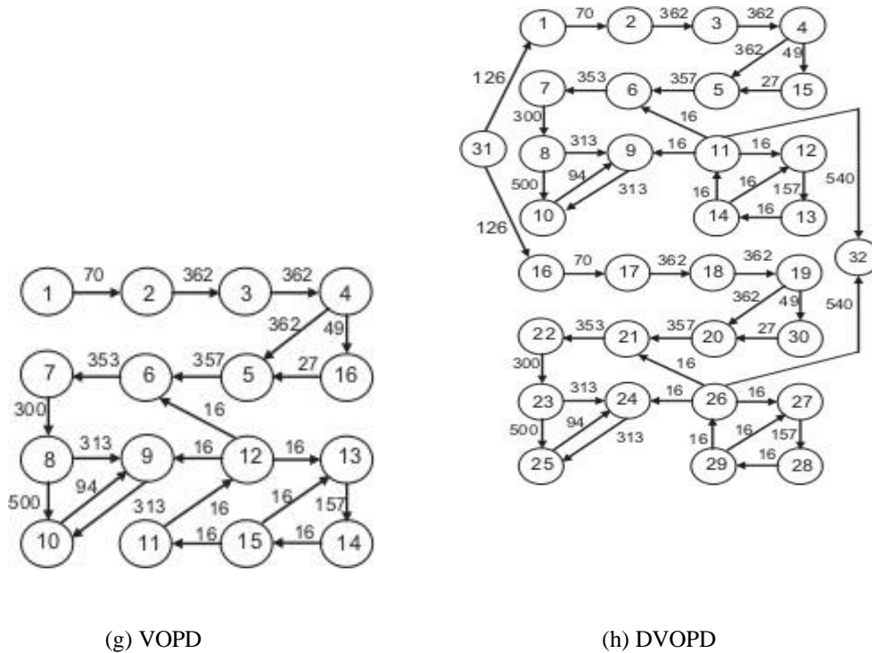
Fig 1. Task graphs 2
