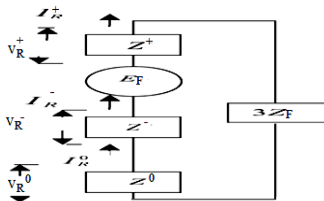
Fig 5. Equivalent circuit (SLG)
