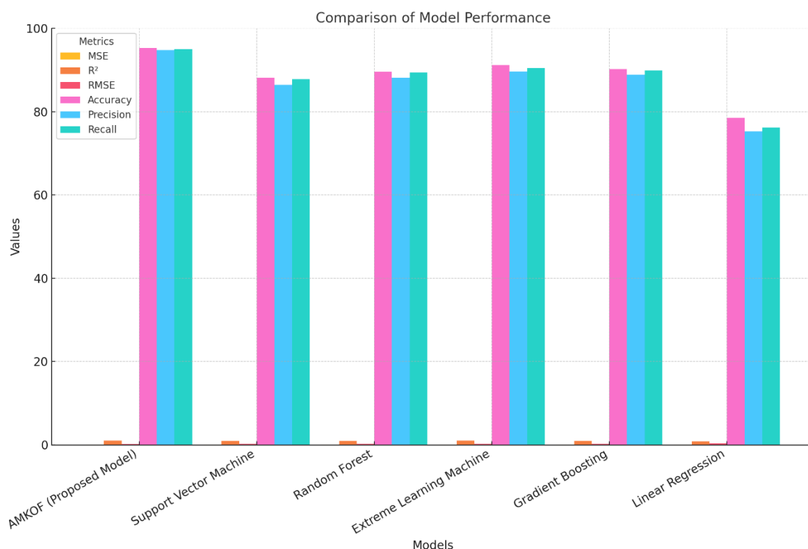
Fig. 2 Bar chart comparing the performance metrics of the AMKOF model against other machine learning models. The AMKOF model demonstrates consistently superior performance across all evaluation metrics.
